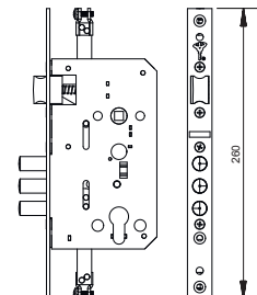
MPL 212 - P/N 26900254
